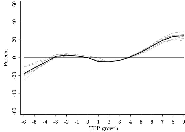
Figure D.21: Hairplots dropping each technology one at a time - Full sample
