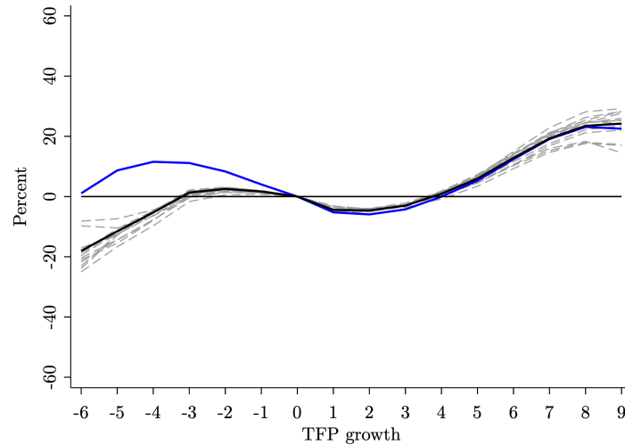
Figure D.23: Hairplots dropping successive 5-year windows each time - Full sample
