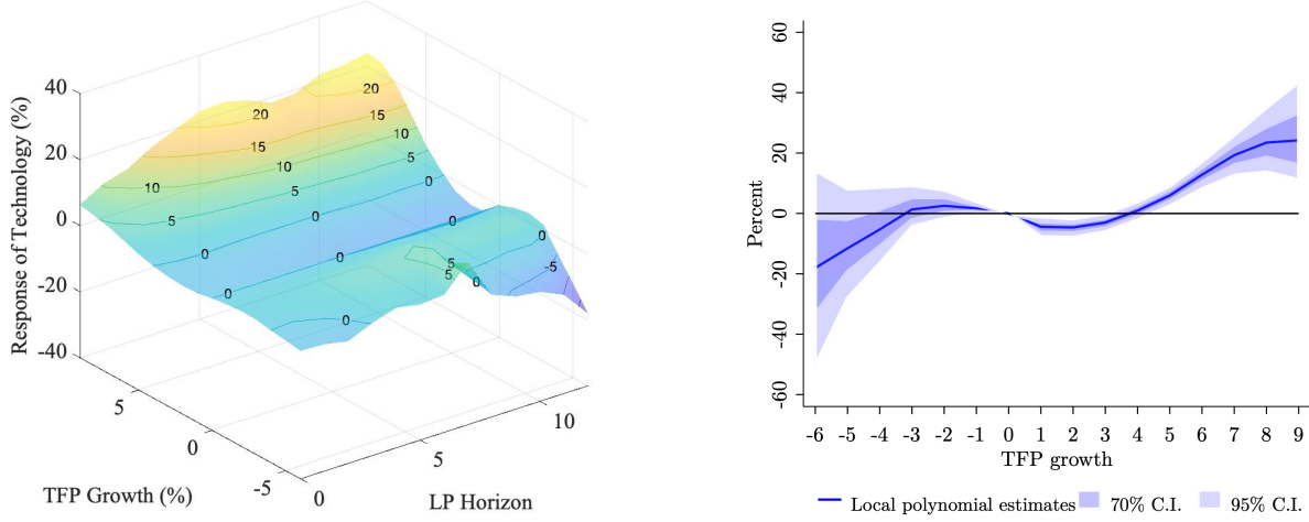
Figure 7: \hat{\mathcal{R}}(h, \varepsilon) - Full sample
